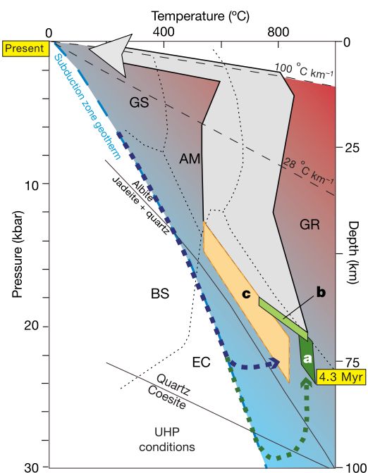
Figure 2 Pressure–temperature conditions for D'Entrecasteaux eclogites. a , This study; b , from ref. 10; c , from ref. 12. Exhumation path based on compilation of P – T data for eclogites, shear zone gneisses, and retrogressed core zone gneisses 13 . Two possible prograde paths for the eclogite are indicated as dashed lines with arrows. Metamorphic facies (abbreviations as in Fig. 1; GR, granulite), coesite = quartz, and jadeite + quartz = albite reaction curves indicated. Mineral compositions are given in the Supplementary Information. Subduction zone geotherm, and present-day range of thermal gradients from the Moresby seamount region 43 , east of the D'Entrecasteaux Islands, are also shown.
