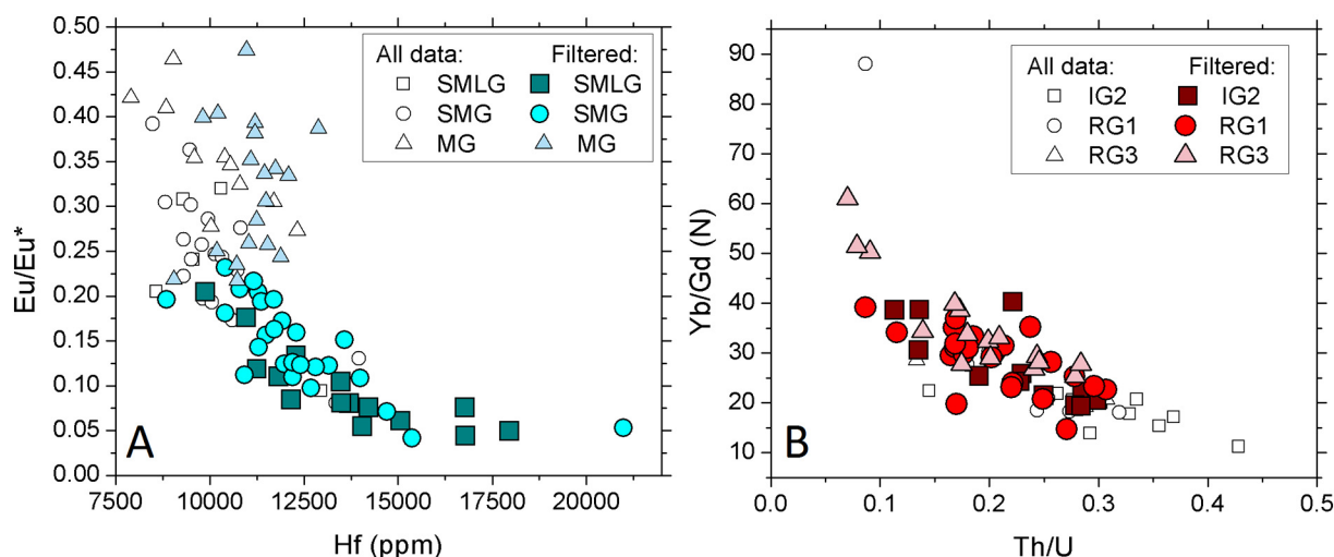
Fig. 10. Application of a conservative LREE-I filter to suites with little evidence for alteration. Filtering out samples with LREE-I < 60 results in negligible changes to interpretations of the early melt history. A) Samples from the Spirit Mountain batholith; B) samples from the youngest pulse of San Jacinto granitoids.
