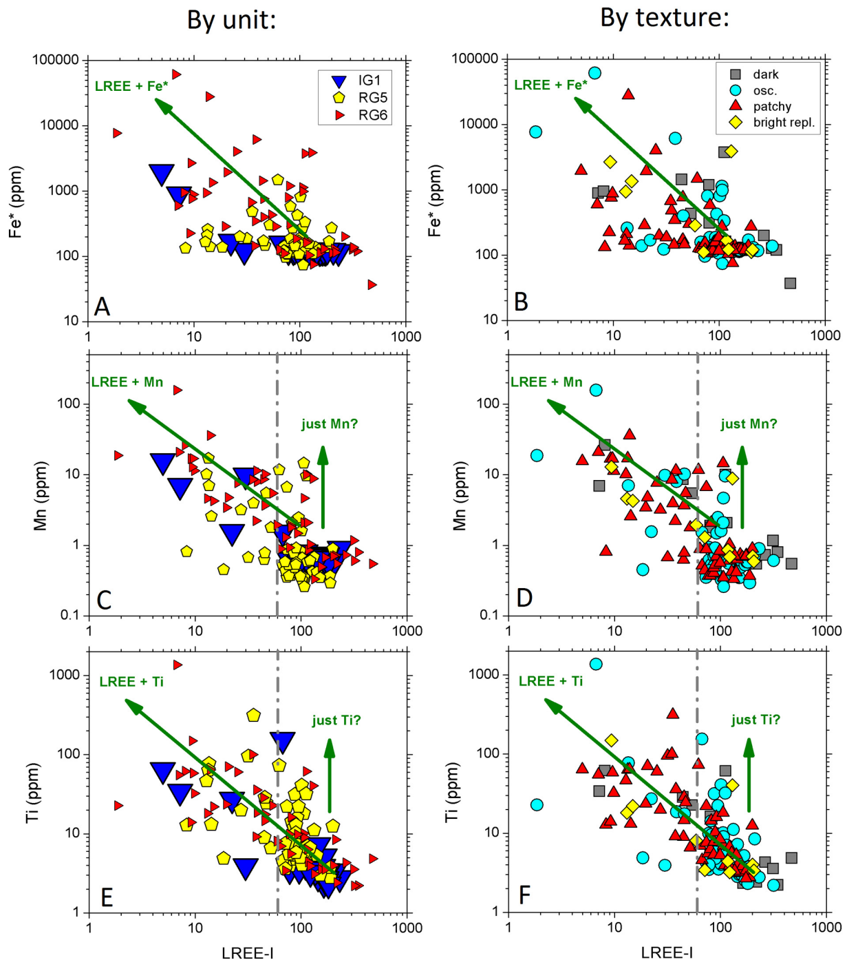
Fig. 6. Relationship between LREE-I and various contaminants in zircon from the older San Jacinto suite. A, C, E) data grouped by unit; B, D, F) data grouped by zircon CL texture. A, B) \text{Fe}^* vs LREE-I reveals contamination involving higher LREE as well as \text{Fe}^* ; C, D) Mn vs LREE-I reveals LREE + Mn contamination as well as potential contamination by Mn without substantial LREE; E, F) Ti vs LREE-I similar to results for Mn. Samples with LREE-I > 60 appear to show negligible LREE alteration.
