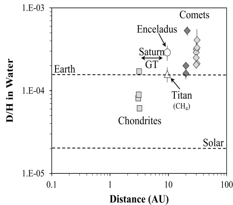
Fig. 5 The H isotopic compositions of OH/water in various objects as a function of radial distance from the Sun (modified after Alexander 2017). The H isotopic composition of methane in Titan's atmosphere is also shown, although it is not known how closely it reflects that of the water that Titan accreted. The locations of the asteroidal parent bodies of the carbonaceous chondrites are not known and so they have been given nominal radial distances of 3 AU. Saturn's moons Titan and Enceladus have been given their current orbital distances, although if there was a Grand Tack they may have formed between \sim 3 AU and \sim 7 AU ( double arrowed ). The formation locations of the comets are unknown, but are thought to have been between \sim 20 AU and \sim 30 AU (e.g., Brasser and Morbidelli 2013). The Oort ( light grey ) and Jupiter family ( dark grey ) comets are plotted at 30 AU and 20 AU, respectively, but their overlapping D/H ratios suggest that they formed in similar regions of the disk. With the possible exception of the CRs, the carbonaceous chondrite with the most D-rich water, the carbonaceous chondrites have compositions that are distinct from any measured outer Solar System body. Data sources are given in Tables 4 and 5
