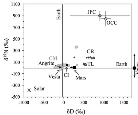
Fig. 7 Comparison of the estimated bulk H and N isotopic compositions of the major inner Solar System bodies with those of the average Jupiter family (JFC) and Oort Cloud (OCC) comets and individual members of the most volatile-rich chondritic meteorites. The H isotopic composition given for Mars is probably an upper limit. The H isotopes of the comets, based on their water compositions, are probably lower limits for their bulk compositions, whereas their N isotopes are probably upper limits (see text for details). Venus has lost almost all of its original water and its initial H isotopic composition is unknown. The sources are given in Tables 5 and 6
