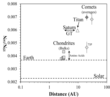
Fig. 6 The same as for Fig. 5 but for N isotopes (modified after Alexander 2017). The N isotopic compositions of individual comets are generally very consistent but the uncertainties can be large (Table 6), so they have been averaged, except for the JFC outlier comet 73P. Titan's atmospheric N isotopic composition is thought to reflect that of the \text{NH}_3 it accreted (Mandt et al. 2014). The carbonaceous chondrite compositions are for bulk meteorites (Table 3). However, amino acids and other N-bearing soluble organic compounds (vertical double arrow) probably formed from \text{HCN}/\text{NH}_3 and exhibit a similar range of isotopic compositions to the bulk meteorites (see text and Table 6 for sources)
