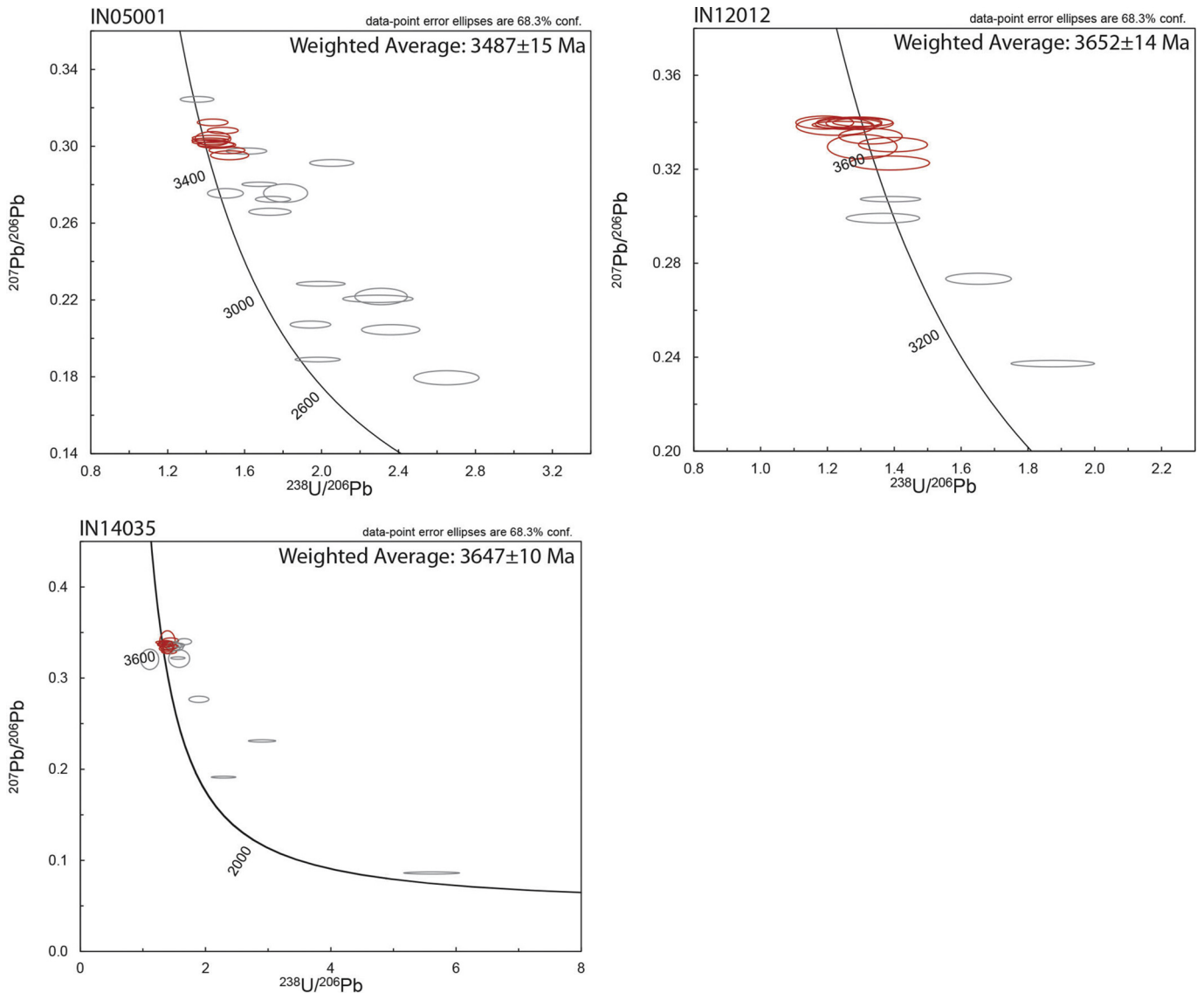
Fig. 10. U–Pb zircon geochronology expressed in Tera-Wasserburg plots for Central Tonalitic Gneiss samples (IN05001, IN12012, IN14035); gray ellipses not included in the weighted average ^{207}\text{Pb}/^{206}\text{Pb} age.
