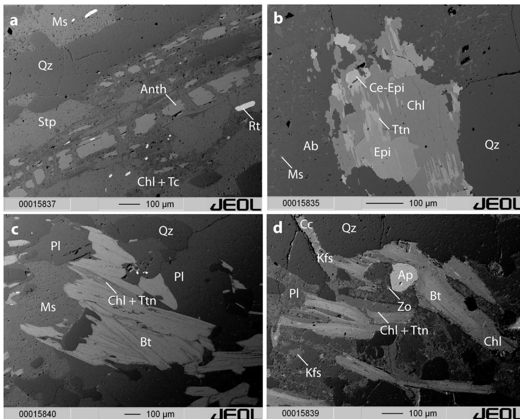
Fig. 6. Back-scatter electron images illustrating the textural relationships in four representative samples discussed in the text. (a) Meta-conglomerate sample IN14032A shows the mineral assemblage anthophyllite (Anth) + muscovite (Ms) + stilpnomelane (Stp) + quartz (Qz) + rutile (Rt). Anthophyllite is replaced by the assemblage chlorite + talc (Chl + Tc). (b) Boizard suite granite sample IN12016 contains the mineral assemblage chlorite (Chl) + epidote (Epi) + titanite (Ttn) + albite (Ab) + quartz (Qz). (c) The gray gneiss sample IN14036 shows the mineral assemblage biotite (Bt) + muscovite (Ms) + plagioclase (Pl) + quartz (Qz). Biotite is replaced by chlorite + titanite (Chl + Ttn). (d) The Voizel tonalite sample IN12044 contains the mineral assemblage biotite (Bt) + K-feldspar (Kfs) + plagioclase (Pl) + quartz (Qz) + apatite (Ap). Biotite is replaced by chlorite + titanite (Chl + Ttn) and albite contains small zoisite (Zo) grains.
