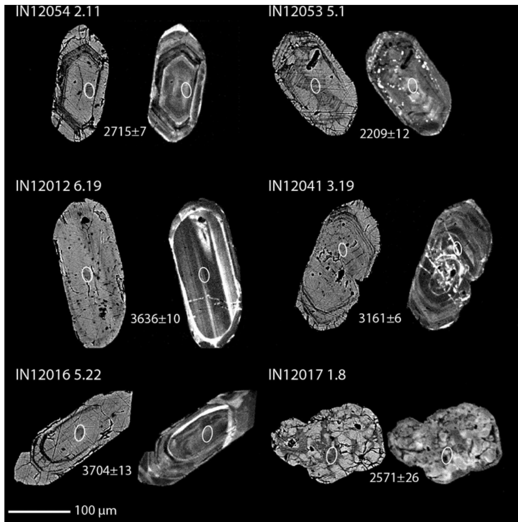
Fig. 5. Back-scattered electron and cathodoluminescence paired images of representative zircon grains reported in this work (a–f). (a) Example of a euhedral, igneous zircon; note rim with bright CL response. (b) Example of an igneous core with an overgrown metamorphic rim. (c) Example of a rounded, inherited core surrounded by an igneous overgrowth. (d) Example of a zircon with a texture typical of metamictization. (e) Zircon with a geochronology spot that has overlapped a fracture. (f) Zircon with a texture that suggests intense metamictization and/or hydrothermal alteration. Please see Supplementary Figs. S1 for the complete documentation of these samples.
