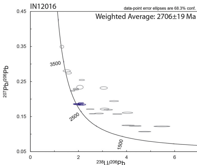
Fig. 12. Boizard suite U–Pb zircon geochronology; gray ellipses not included in weighted mean ^{207}Pb/^{206}Pb age.
