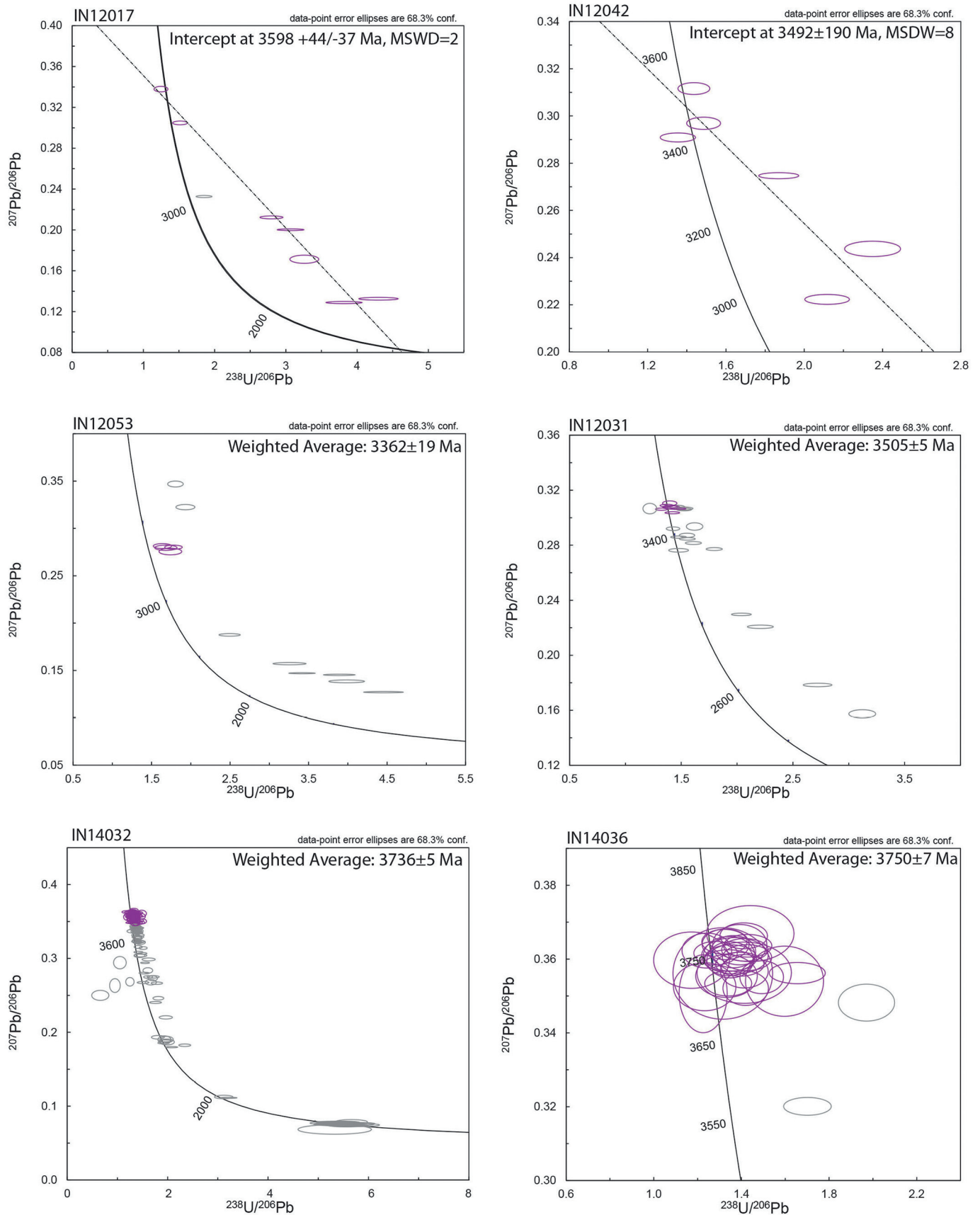
Fig. 13. U–Pb zircon geochronology for various supracrustal (NSB and USB) and USB intrusion samples; gray ellipses not included in weighted mean or upper intercept age calculations.
