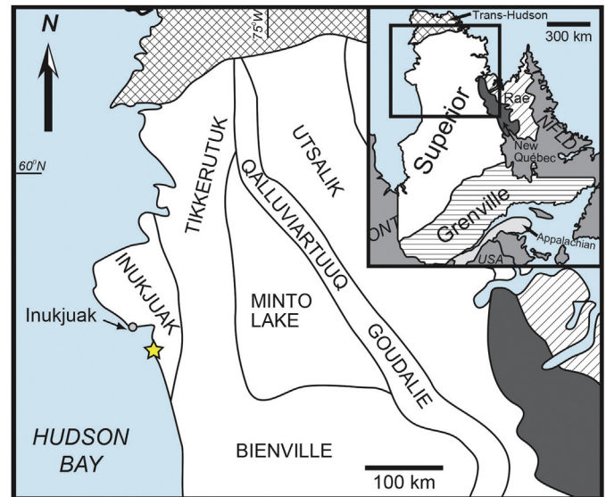
Fig. 1. Simplified map of the northwestern Superior Province, with the location of the town of Inukjuak (gray dot) and the study area (yellow star) highlighted.
