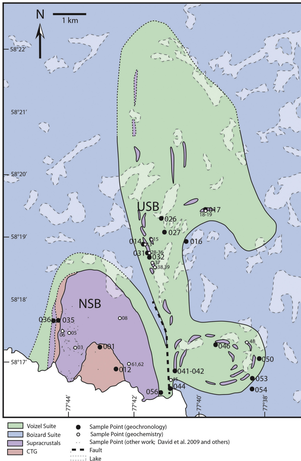
Fig. 3. Local geologic map showing the main lithologies discussed herein. Samples described in this work are represented by large black dots, additional samples with geochemical data are represented by small white dots, and samples from other studies are represented by small gray points (see Supplementary Information in Cates et al., 2013 for reported data tables).
