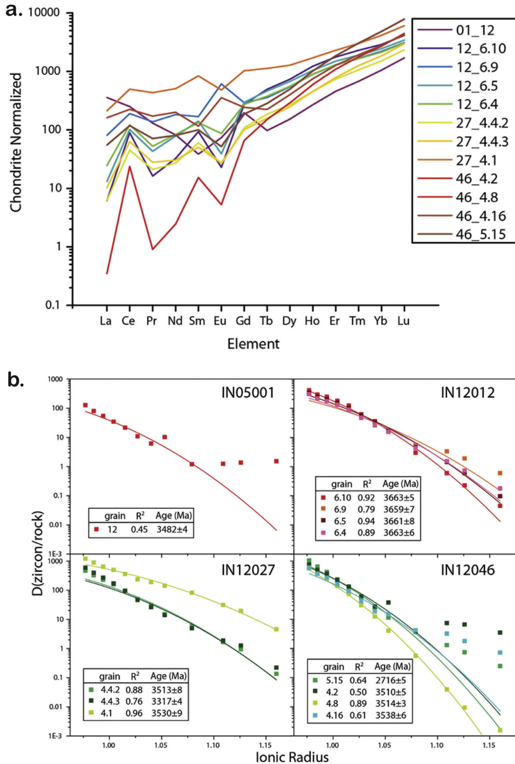
Fig. 14. (a.) REE data plotted for zircons used in the lattice-strain partitioning modeling work described herein. (b) Onuma diagrams of selected zircons from TTG and Voizel samples showing R 2 fitting values (see Mojzsis et al. 2014 and references therein). Colors correspond to the calculated partition values for a particular grain using its host rock, and the model best-fit line.
