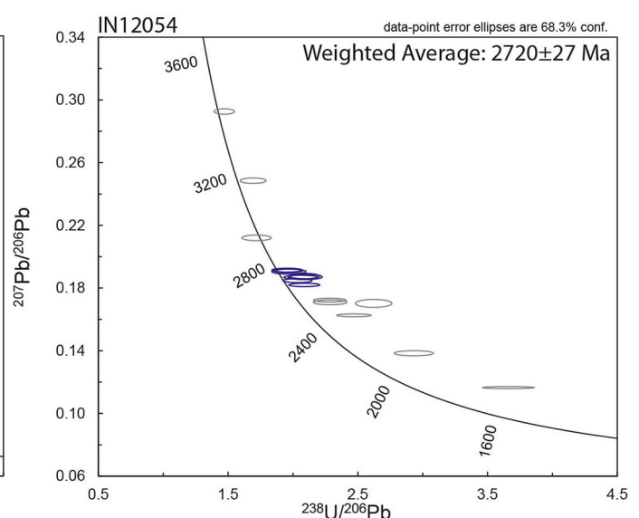
Fig. 12. Boizard suite U–Pb zircon geochronology; gray ellipses not included in weighted mean ^{207}Pb/^{206}Pb age.
