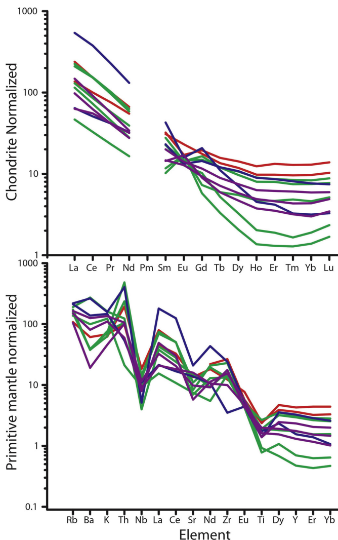
Fig. 8. (top) Chondrite-normalized (Anders and Grevesse, 1989) REE plot; (bottom) Primitive Mantle-normalized (McDonough, 1992) multi-element plot. Color coding of the samples as in Fig. 7 (Supplementary Table S1).
