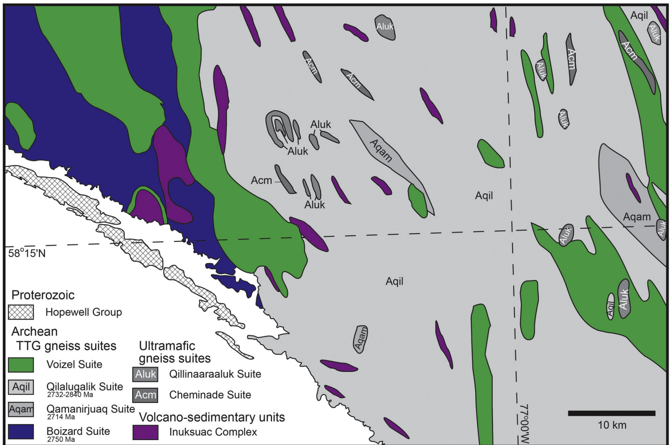
Fig. 2. Regional geologic map (after Simard, 2003) showing the geological context of the ancient supracrustal remnants of the Innusuaq Complex. The study area is outlined by the rectangle (see Fig. 3). Rock suites that have not been substantially characterized are shown in gray.
