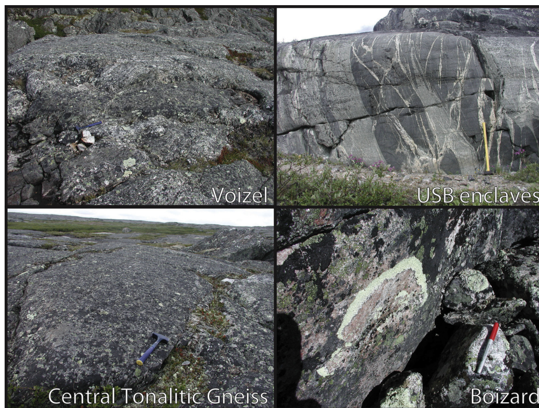
Fig. 4. Field photographs of the main lithologies discussed in this work. The Voizel suite is represented by sample IN12041 (hammer for scale, ~30 cm); Ukaliq enclaves are exemplified by sample IN12042 (as a white gneiss that cross-cuts amphibolite; 1 m hammer for scale); an example of the Central Tonalitic Gneiss is from sample IN12012 (hammer for scale); and the Boizard suite is represented by IN12054 (pen for scale, 10 cm). (For interpretation of the colors in this figure, the reader is referred to the web version of this article.)
