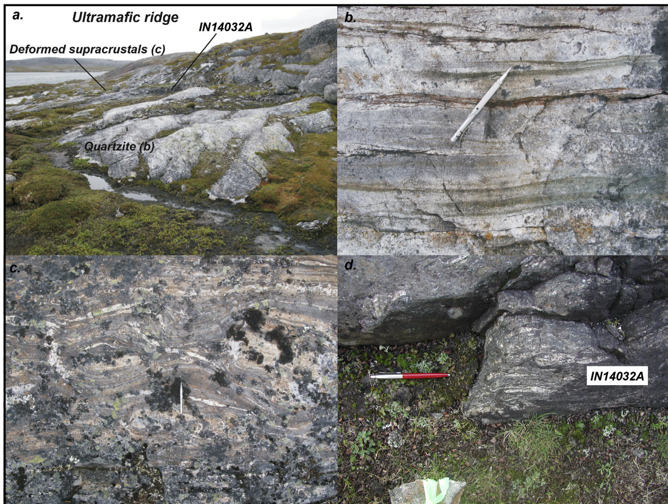
Fig. 9. (a) Light-colored quartz-rich rocks below the belt of ultramafic boudins in the northern Ukaliq supracrustal belt. Significantly, the quartz-rich rocks appear to show a progression from detrital quartzites to meta-cherts with magnetite-bearing laminae higher up. Sample location of IN14032A is annotated in the figure. (b) Close-up view of the quartz-rich rocks of probable detrital origin (i.e. quartzite proper). Note subtle aspects of the relict layering suggesting both grading and truncations. The greenish color is probably due to calc-silicates. (c) Mesoscopic view of highly deformed amphibolites and supracrustal gneiss, with strong boudinage of the more competent layers. Gneissosity has been pulled into the boudin necks and folded, whereas quartz-feldspar veins and pods fill discontinuities and areas of strong local extension. (d) Quartz-biotite schist at the base of the ultramafic body (IN14032A; labelled) for which detrital zircon U–Pb geochronology was attempted. These various outcrop-scale structures illustrate the structural style of the Ukaliq supracrustal belt, with the boudins being analogous to the larger ultramafic bodies in the wider area, and the quartz veins representing late Neoproterozoic granitic pegmatites that intruded late during the boudinage forming deformation. (For interpretation of the references to color in this figure, the reader is referred to the web version of this article.)
