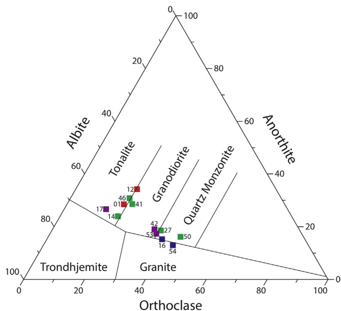
Fig. 7. Classification of samples based on normative anorthite, albite, and orthoclase compositions. Fields from Barker (1979). CTG samples are red, Voizel samples are green, Boizard samples are blue, and supracrustals and USB enclaves are purple. Numbers refer to the last two-digits of the sample identifiers in Supplementary Table S1.
