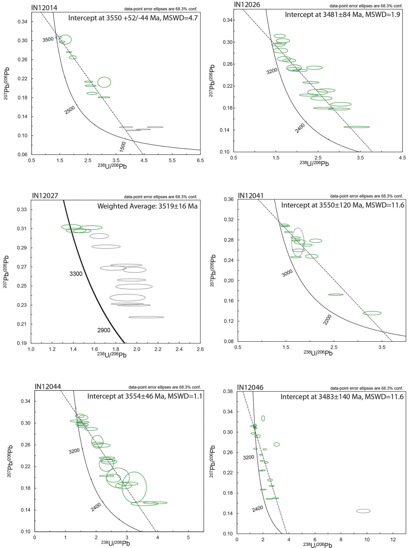
Fig. 11. U–Pb zircon geochronology for Voizel suite samples investigated in this work; gray ellipses not included in weighted mean or upper intercept age calculations.
