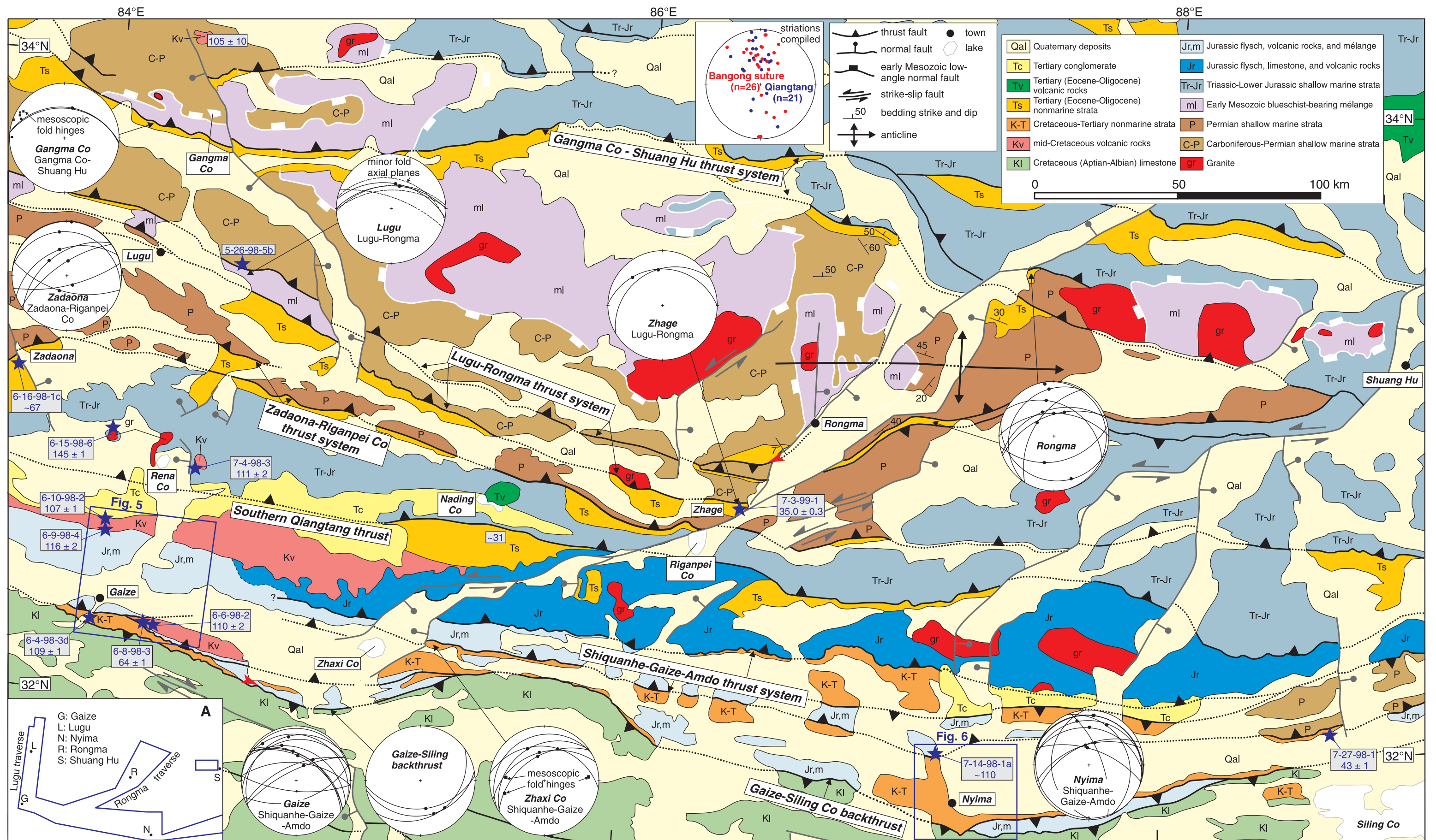
Figure 2. Geologic map of central Tibet. (A) Inset shows areas that have been mapped at 1:100,000 scale (Kapp et al., 2003b; this study). The geology between map areas is based on our interpretations of satellite imagery and 1:1,000,000-scale (Cheng and Xu, 19886) and 1:1,500,000-scale (Liu, 1988) geologic maps. Structural measurements are plotted on lower hemisphere equal-area stereonets. Blue stars show geochronologic sample localities with sample numbers and interpreted crystallization ages (in Ma and analytical uncertainties at 2\sigma ). Stratigraphic age assignments, if not constrained by our studies, were based on correlating observed lithostratigraphy with nearby biostratigraphic sections (Cheng and Xu, 19886; Li and Zheng, 1993; Li et al., 1995) and should be considered tentative.
