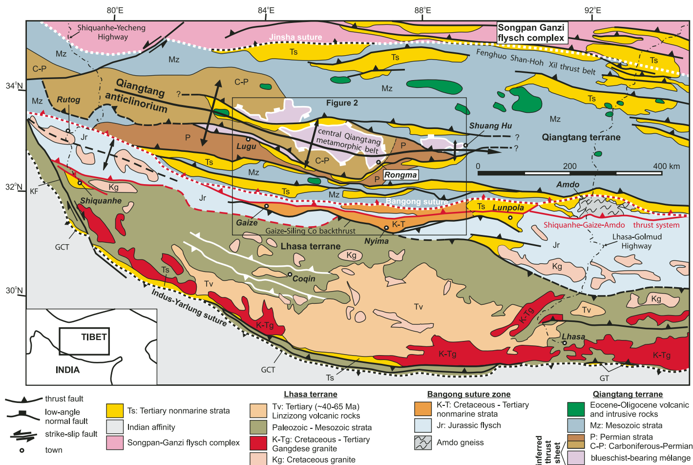
Figure 1. Tectonic map of southern and central Tibet modified from Kapp et al. (2003a). Tertiary thrust faults are shown in black. Major Mesozoic faults are shown in white: the Coqin thrust belt of Murphy et al. (1997) and early Mesozoic domal low-angle normal faults in the central Qiangtang terrane (Kapp et al., 2000, 2003b). Abbreviations: GCT—Great Counter thrust; GT—Gangdese thrust system; KF—Karakoram fault.
