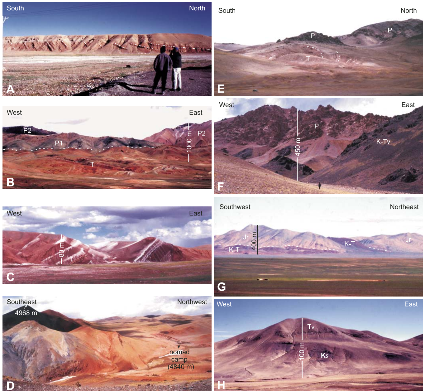
Figure 7. (A) Synorogenic nonmarine strata near Nyima (Fig. 5) as indicated by the northward fanning of dips toward shallower angles along the south limb of a syncline. The red beds are overlain by Neogene-Quaternary(?) fluvial conglomerate. (B) North-dipping thrust fault near Zhage (Fig. 2), which juxtaposes Permian volcaniclastic sandstone and turbidites (P1) and conformably overlying limestone (P2) in the hanging wall against Tertiary red beds in the footwall. (C) Gypsiferous Tertiary basin fill in the footwall of the Lugu-Rongma thrust system near Zhage (Fig. 2). (D) Southeast-dipping backthrust associated with the Lugu-Rongma thrust system near Rongma (Fig. 2), which places early Mesozoic mélangé over Tertiary red beds. (E) Gently north-dipping thrust fault near Zadaona (Fig. 2) juxtaposing Permian limestone (P) in the hanging wall against Tertiary red beds in the footwall, which are deformed into an overturned syncline. (F) North-dipping thrust fault near Zadaona (Fig. 2) placing Permian limestone (P) on top of overturned Cretaceous-Tertiary volcanic rocks (K-Tv). (G) Imbricate north-dipping thrust faults ~15 km northwest of Nyima (Fig. 6), which repeat Jurassic (Jr) in the hanging wall and Cretaceous-Tertiary(?) red beds (K-T) in the footwall. (H) Broadly folded ca. 64 Ma volcanic tuffs (Tv) unconformably overlying more steeply dipping mid-Cretaceous red beds (Ks) near Gaize (Fig. 5).
