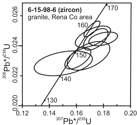
Figure 4. U-Pb concordia plot showing results of single spot ion-microprobe analyses on zircon from a granite near Rena Co (Fig. 2). Error ellipses are shown at the 2\sigma level. Details of the U-Pb method and tabulated results are available in the data repository.
