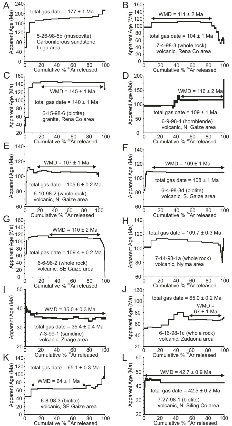
Figure 3. ^{40}\text{Ar}/^{39}\text{Ar} apparent age spectra. Uncertainties for total gas dates and weighted mean dates (WMD) are at the 1\sigma and 2\sigma level, respectively, and do not include uncertainties in the J factor or decay constants. Details of the ^{40}\text{Ar}/^{39}\text{Ar} method and tabulated results are available in the data repository, DR1 [see footnote 1].
