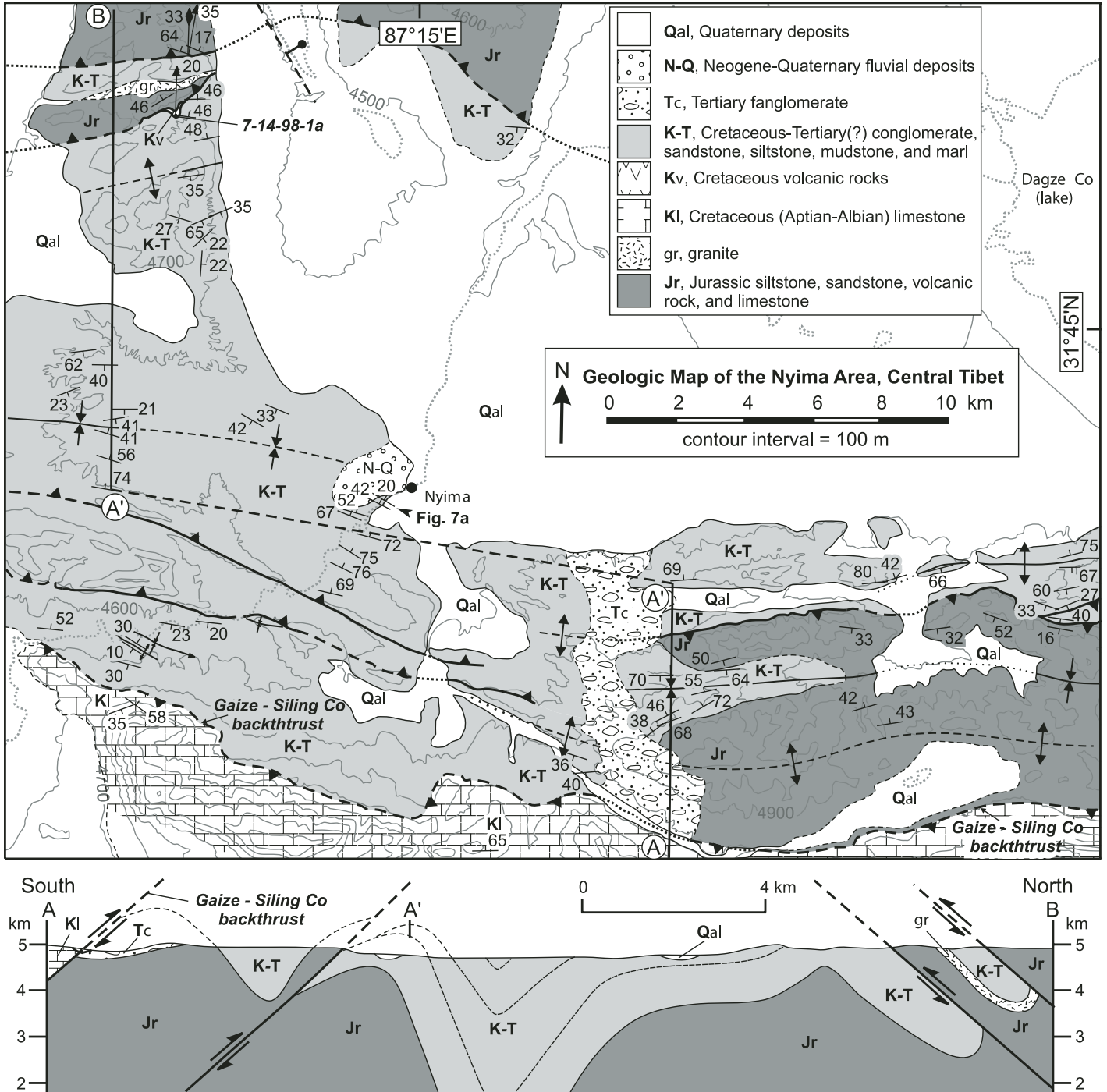
Figure 6. Geologic map and cross section of the Nyima area.
