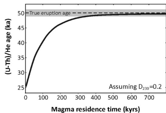
Fig. 1. The effect of magma residence time (x-axis) on measured (U-Th)/He age. The curve is calculated for a zircon crystal with true eruption age of 50 ka by assuming D_{230} = 0.2 which is a typical value for zircon (Charlier and Zellmer, 2000; Farley et al., 2002). The grey band is a typical analytical uncertainty for the (U-Th)/He method. Note that ignorance of a disequilibrium effect may result in underestimation of the age by up to 50% for crystals with short magma residence times. Also note that after >300 kyrs of magma residence, the effect of disequilibrium on (U-Th)/He may not be detectable.
