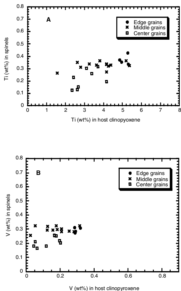
Fig. 9. a) Plot of Ti (wt%) in spinel to the Ti (wt%) of adjacent host clinopyroxene from Leoville 3537–2. Although there is significant scatter, a positive trend is observed; b) Plot of V (wt%) of spinel to V (wt%) of host clinopyroxene in Leoville 3537–2 showing a slight positive correlation. The crystallization sequence of clinopyroxene is from right to left with decreasing Ti in clinopyroxene, the first formed having the highest Ti values. The error associated with each analysis is approximately the same size as the symbols. If error bars are plotted, many of the differences between data points become obscured, thus we have not shown these.
