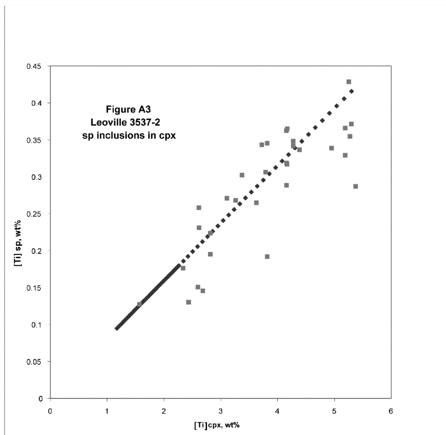
Fig. A3. Comparison of predictions of the Constant D model for spinel inclusions in Leoville 3537-2 clinopyroxene compared with measured Ti concentrations in spinel and clinopyroxene. See Table A3 for parameters. The model is successful in describing both TS-34 and Leoville with the same adopted spinel and clinopyroxene Ti crystal-liquid partition coefficients. In this model, melilite appears around 2.3% Ti in clinopyroxene (29% crystallization) and the liquid, spinel, and clinopyroxene concentrations vary slowly after this. Most spinel inclusions in clinopyroxene should have low Ti concentrations, but this is not observed.
